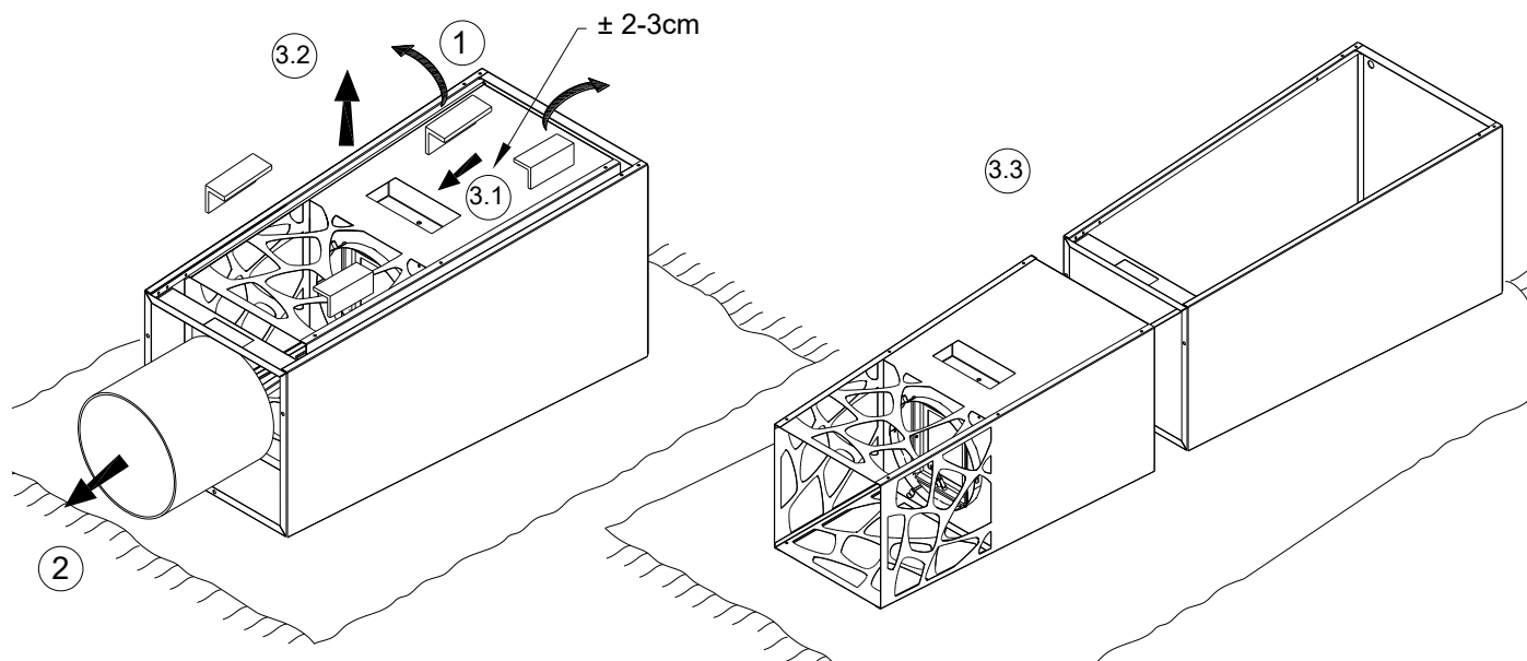
Fig. 5 – Unboxing the fireplace
