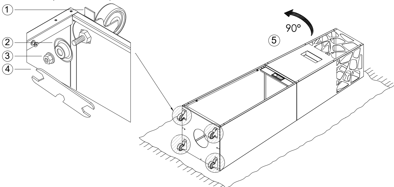
Fig. 7 – Installing the wheels
