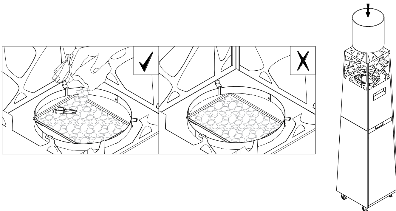
Fig. 8 – PYRAMID top view with ignition elements detail
