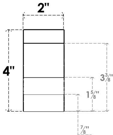
FRONT PROFILE
