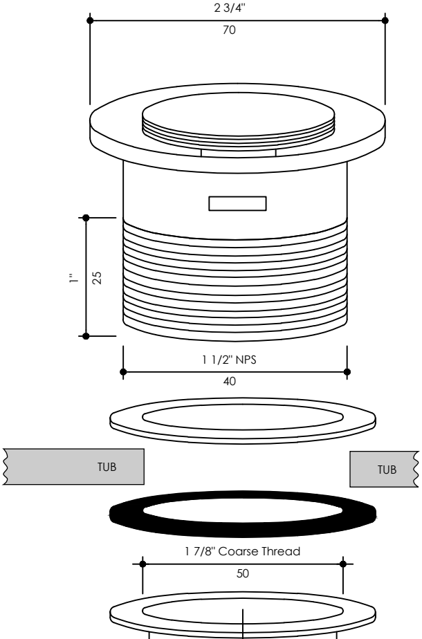
Tub shoe and P-trap connections. Suggested pipe is 1-1/2" diam
