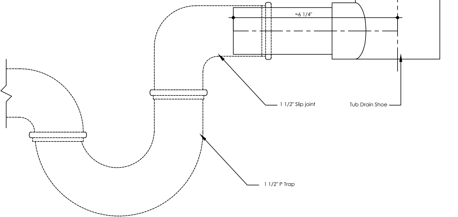
Drain connections.
