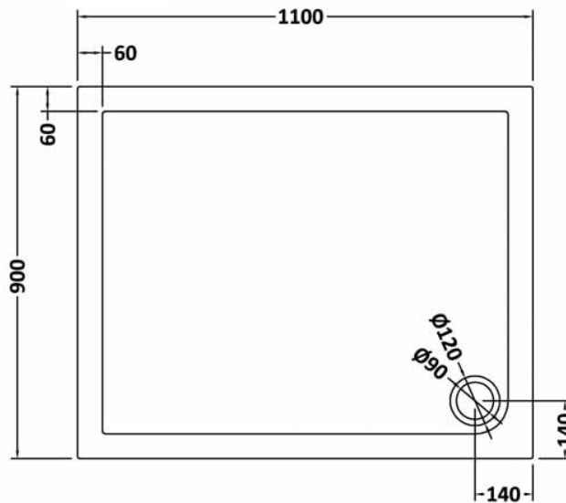
1100 x 900 RECTANGULAR TRAY
