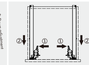
Up & Down adjustment \pm 1.5\text{mm}
