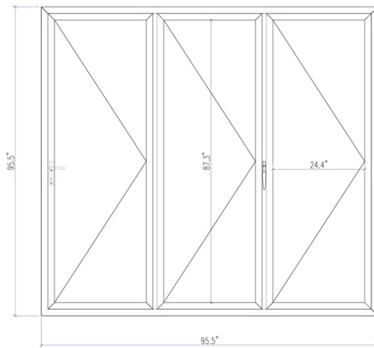
Front View Dimension
