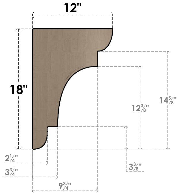
SIDE PROFILE
