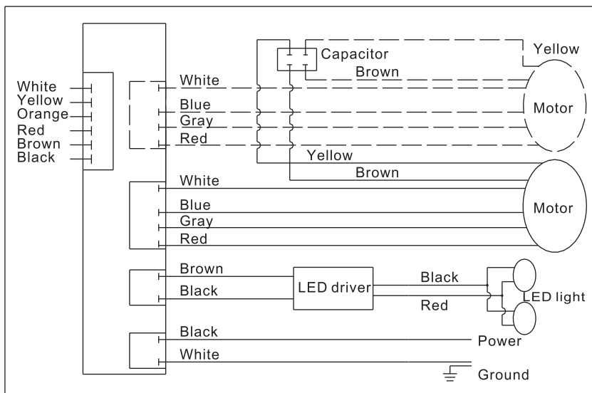
Fig.22 Electrical Schematic Diagram
