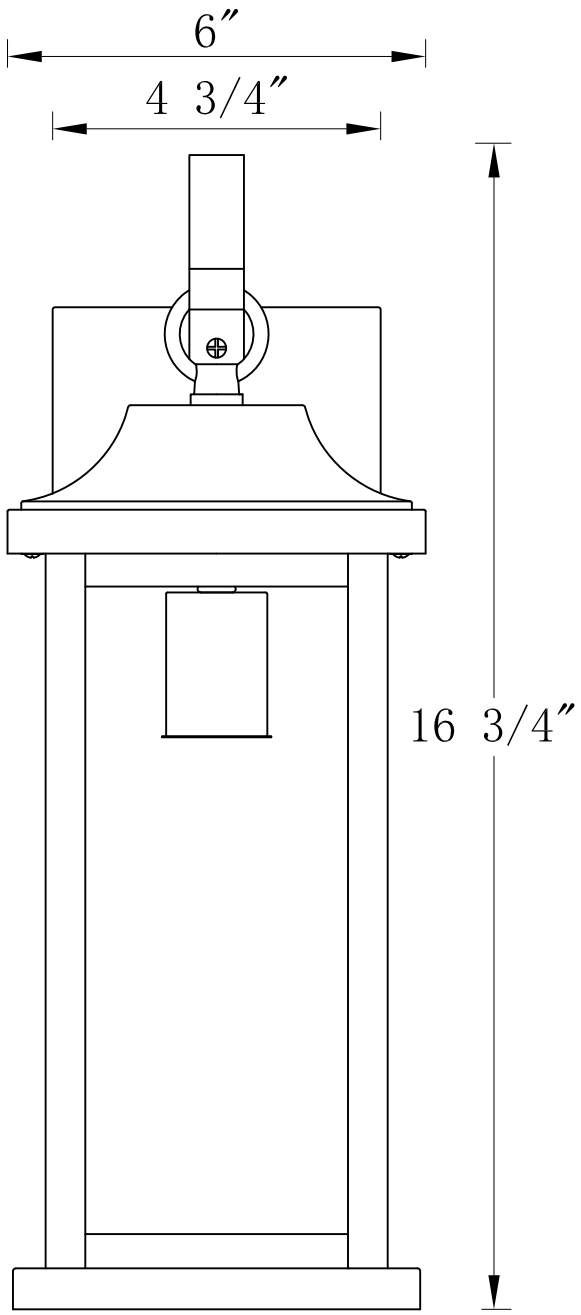
FRONT VIEW
