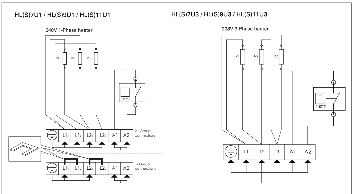
Figure 6. Electrical connections of heater
