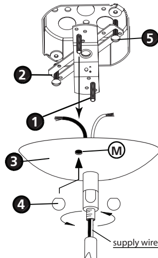
Drawing 3 – Mounting Detail
