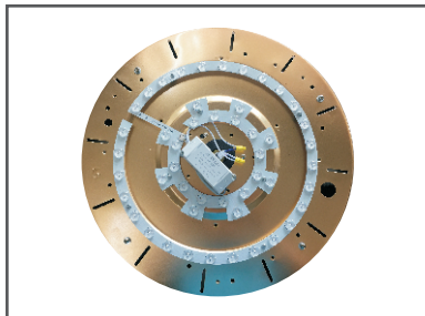
Step 2. The LED light source and LED driver are mounted on the chassis by means of magnets.
