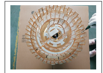
Step 9. Install and fix the lampshade on the chassis with screws.
