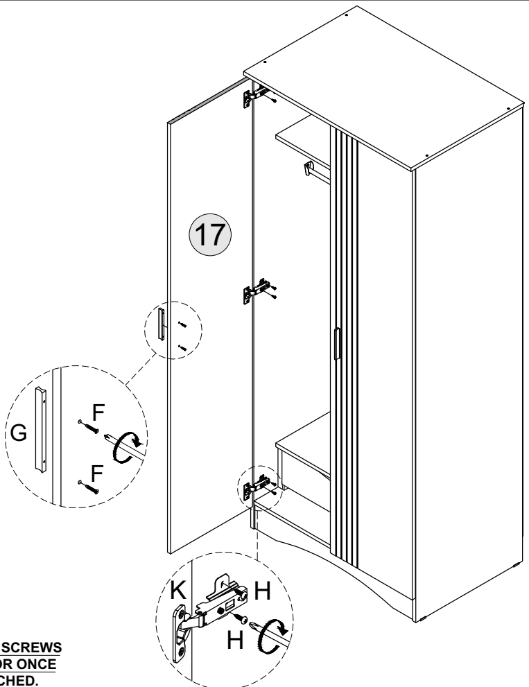
2. LATERAL ADJUSTMENT BY SCREW ADJUSTING
