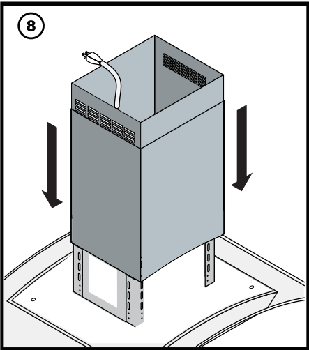
(8) Slip on the chimney over the support frame extensions while ensuring the power cord also slips through.
