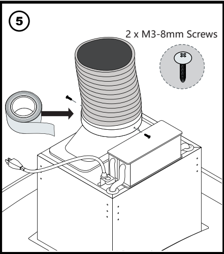
(5) Secure the duct to the vent adapter and use aluminum foil tape to secure a proper seal. (tape not included)
