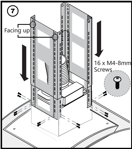
(7) Insert the support frame extensions into the corner brackets (embossed screw holes facing up), and secure them to the range hood with screws.
