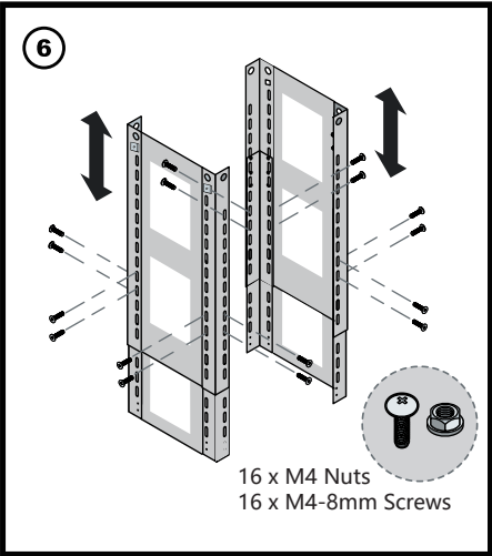
(6) Adjust all support frame extensions to the same required height. Secure each with screws and locking nuts.
