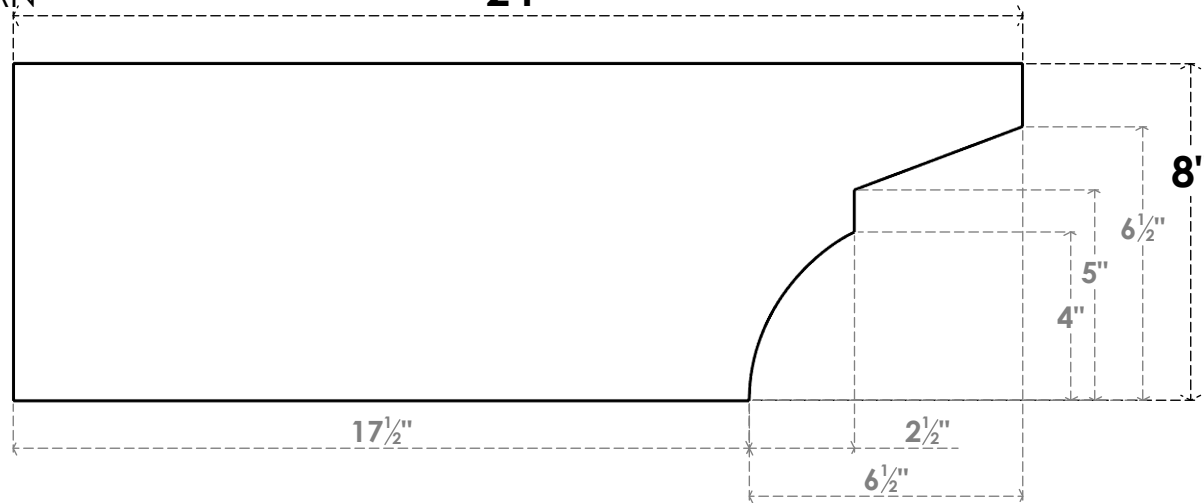
SIDE PROFILE
