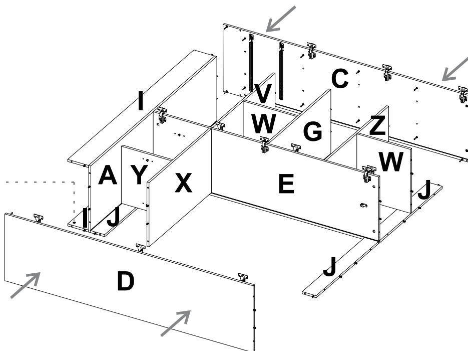
Full Overlay Hinge Bisagra Parche
