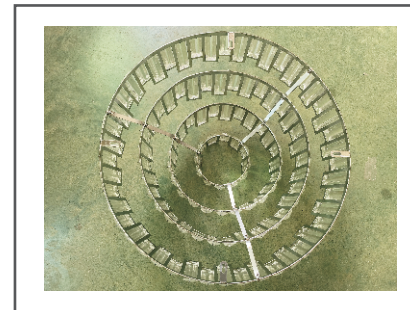
Step 8. Secure the lampshade in turn with the connecting rod.
