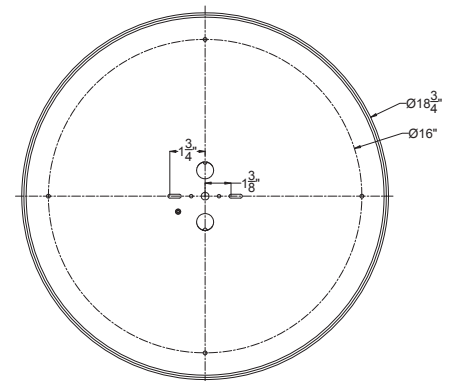
Back Plate
