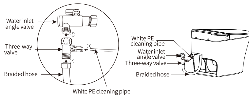
(1) Installation Diagram
