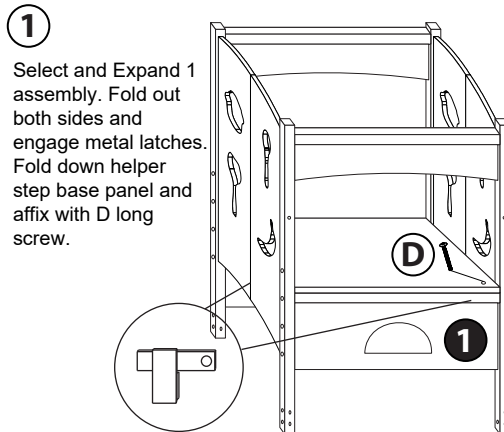
1 - Helper Assembly x1
