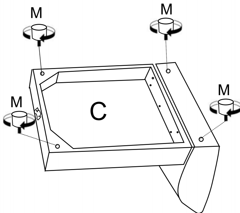
DIAGRAM 6 (Assemble the Legs) Tighten 4 Legs (Parts M) as shown.
