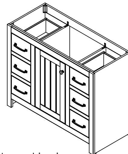
Isometric view
