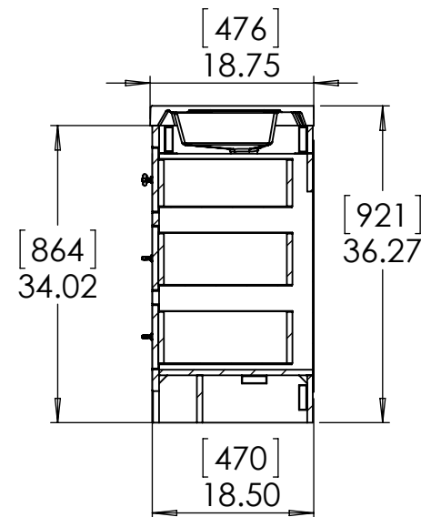
SECTION C-C Side View
