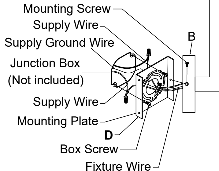
FIG.2 FIXTURE WIRES Black or Smooth
