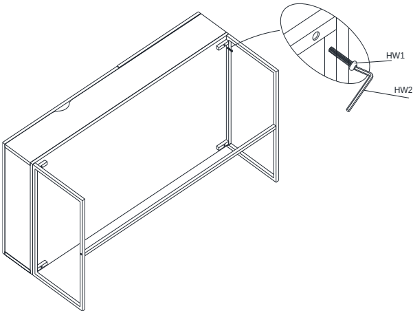
STEP2 assemble the metal frame with the body
