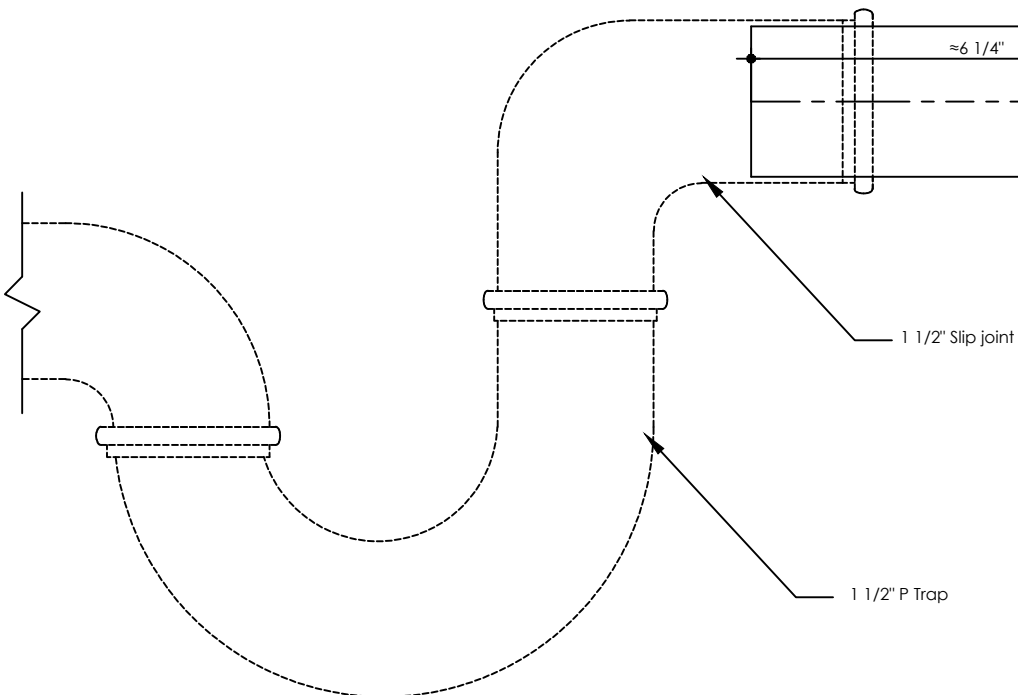
Drain connections.
