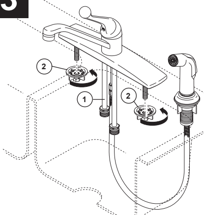
Deck Mount
