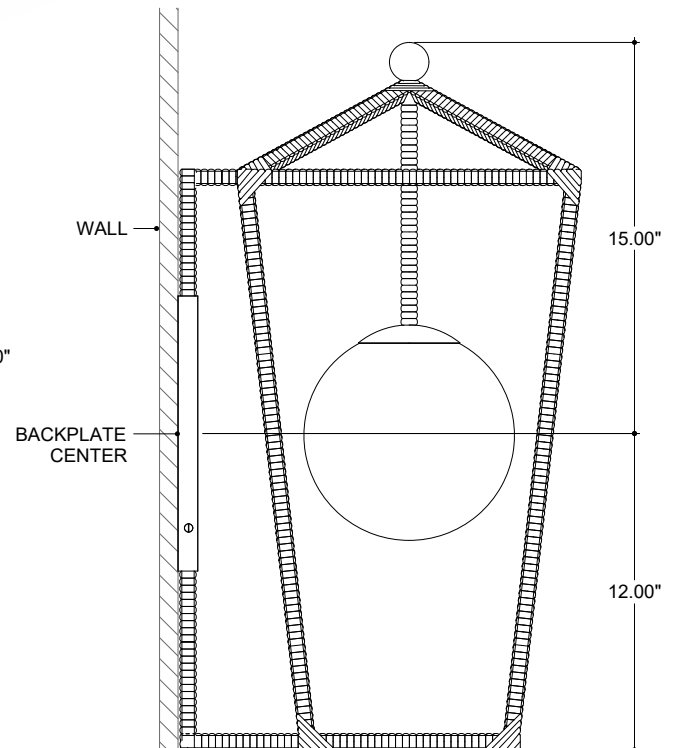
SIDE VIEW
