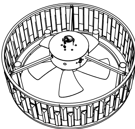
Motor Assembly(1)
