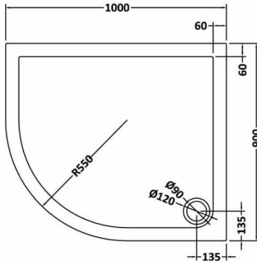
1000 x 900 OFFSET QUADRANT TRAY LH
