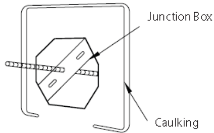
Fig.3 Sealing
