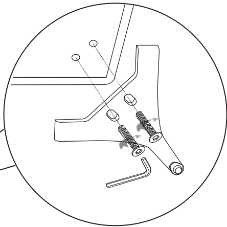
Use allen key to tighten
