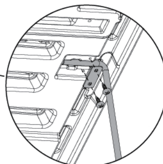
Support rod fixing piece GS0201021
