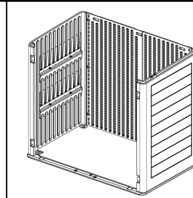
Right back panel BGS08003
