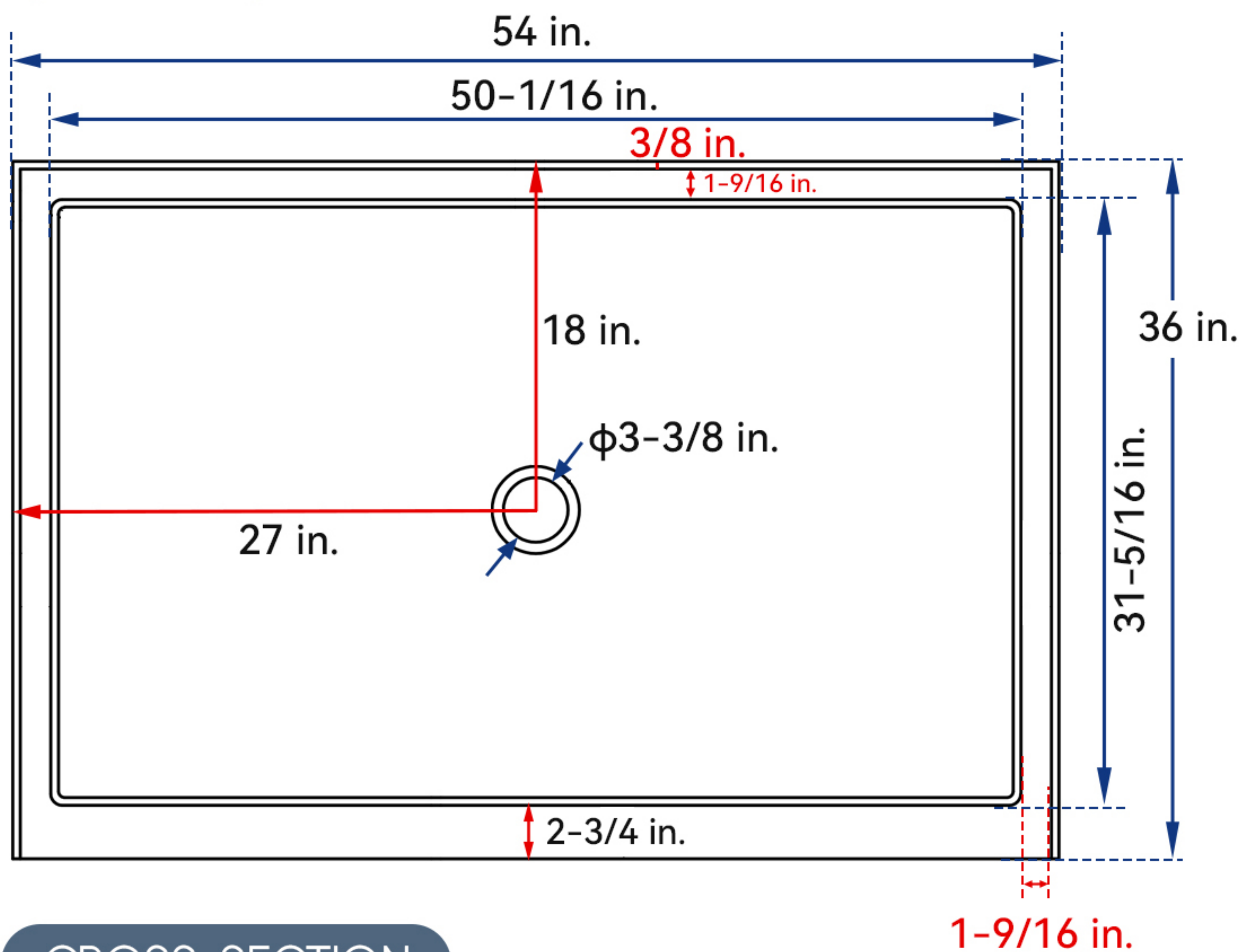
TOP VIEW
