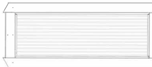
WA09 WINDOW ASSEMBLY - W2A04378 (x1) 1 7/16"x15 1/4"x35 1/4" (36x388x896)
