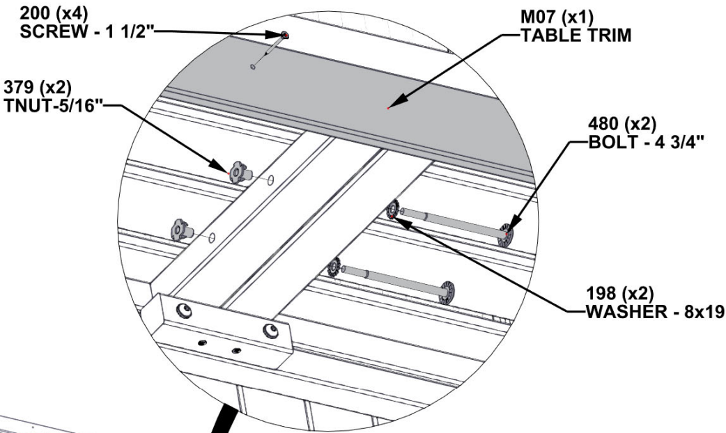
M07 TABLE TRIM - W4L20323 (x1) 5/8"x3 3/8"x44 1/2" (16x86x1131)
