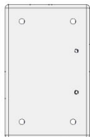
K04 LATCH BLOCK - W4L19789 (x2) 5/8"x3"x4 3/4" (16x76x120)
