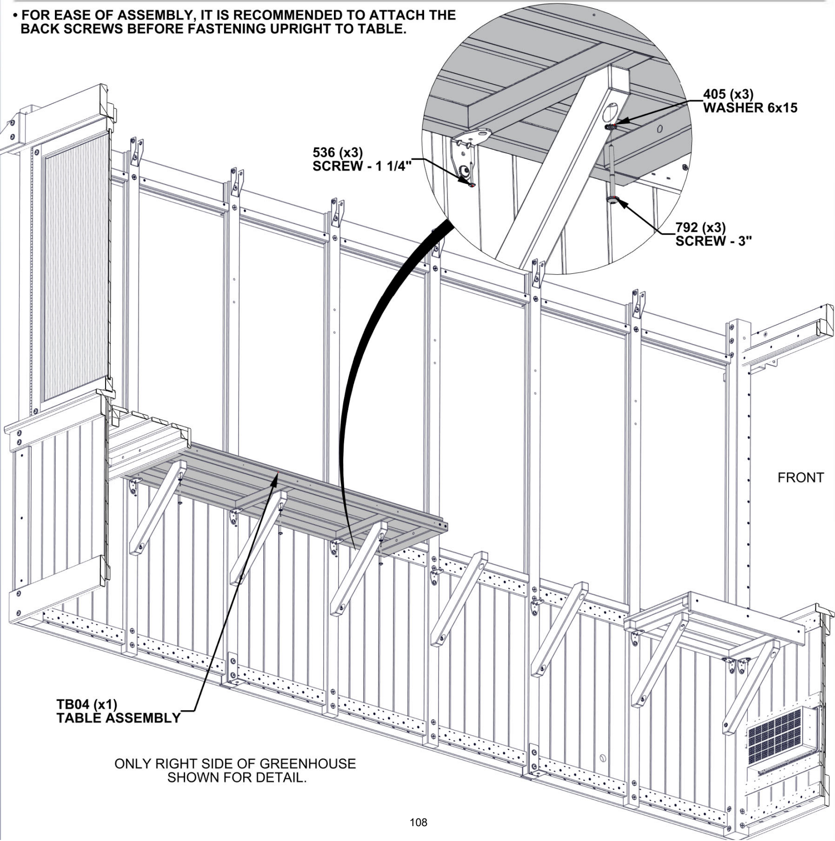
TB04 TABLE ASSEMBLY - W2A04388 (x1) 2 1/16"x16 1/16"x58 7/16" (52x408x1484)
