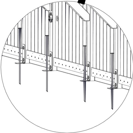
2091 (x12) GROUND STAKE
