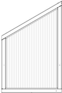
WA04 WINDOW ASSEMBLY - W2A04377 (x1) 1 7/16"x22 3/16"x33 15/16" (36x563x788)
