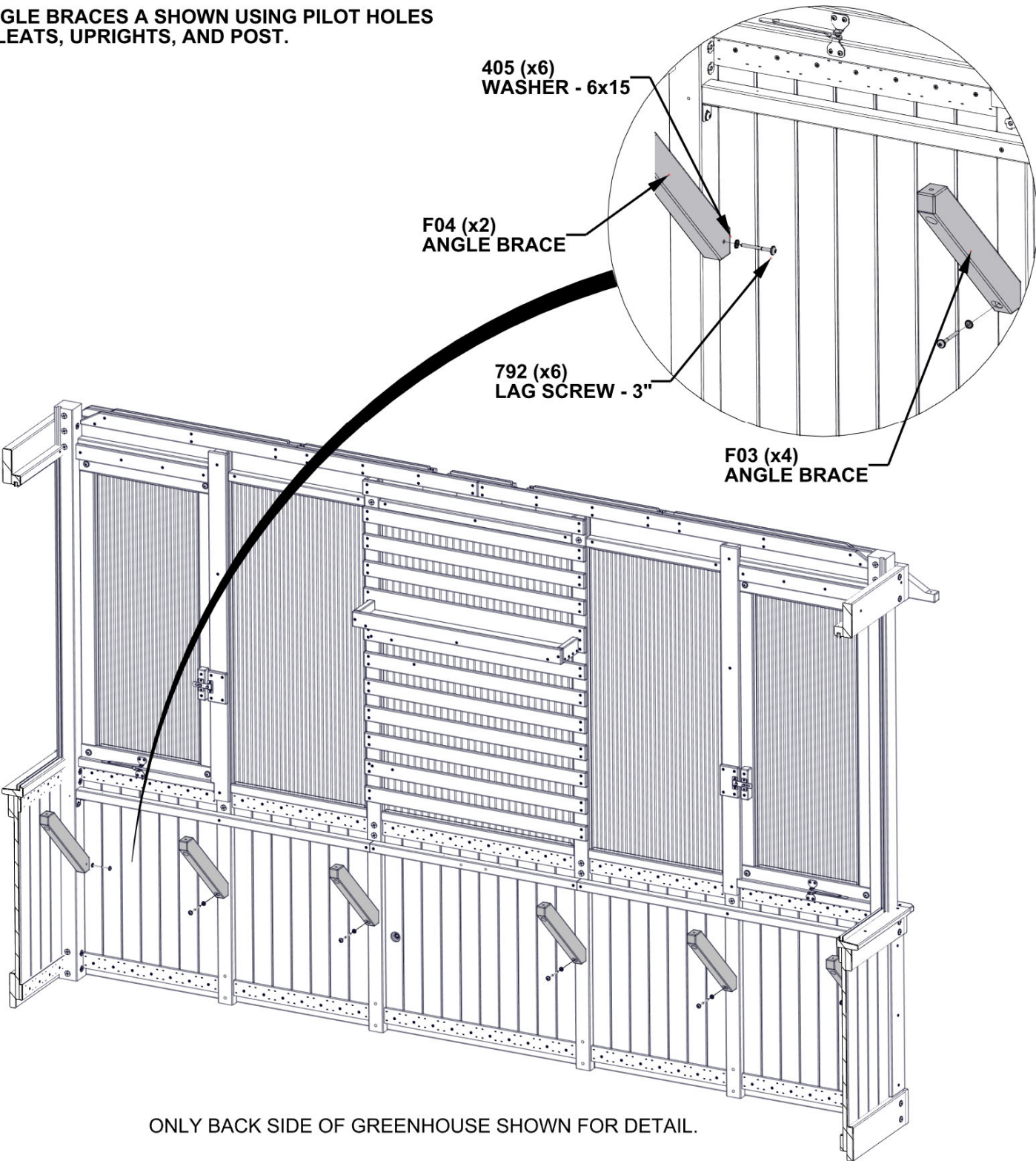
F03 ANGLE BRACE - W4L19487 (x4) 1 7/16"x2 3/8"x18 1/16" (36x60x458)
