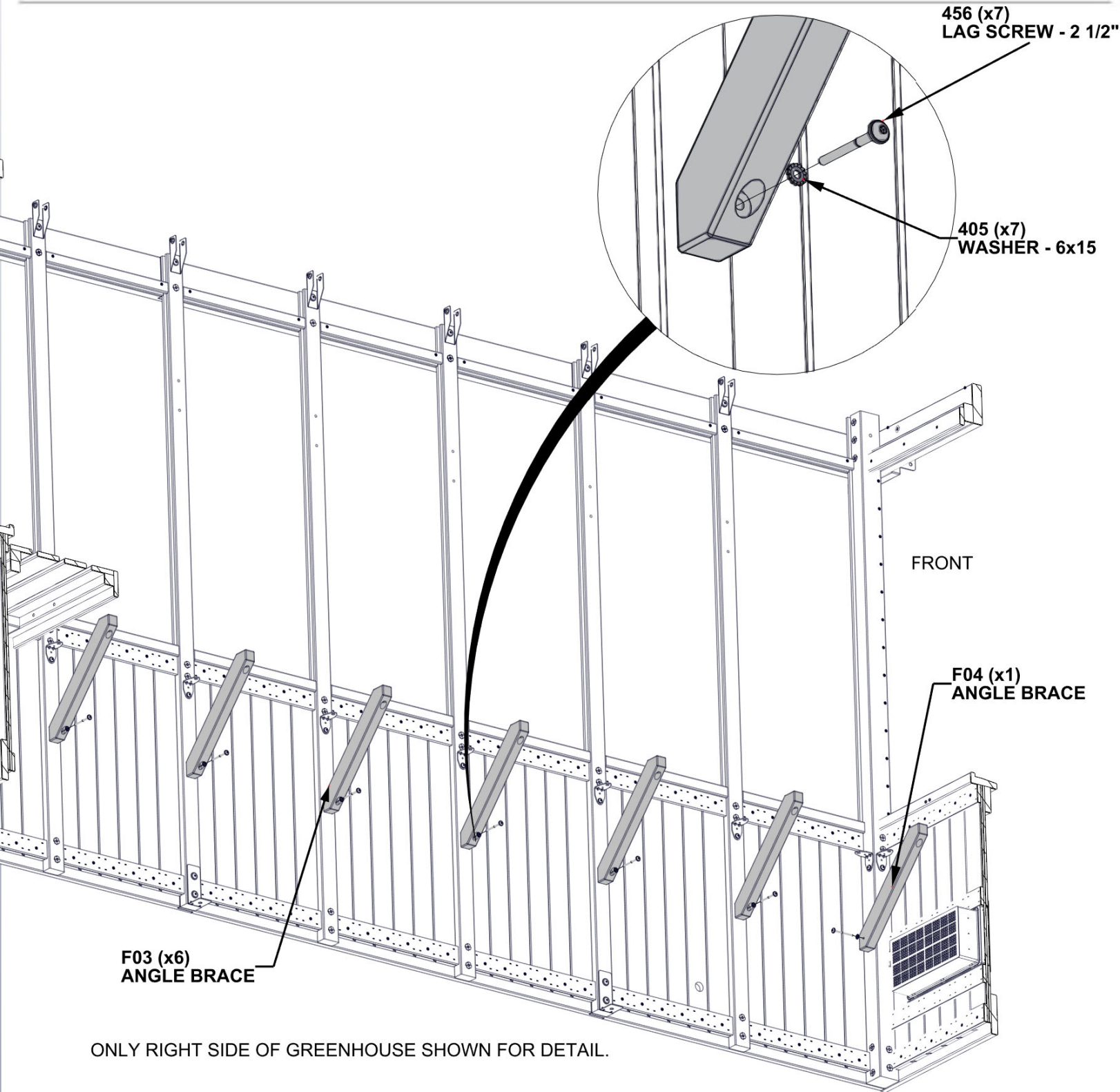
F03 ANGLE BRACE - W4L19487 (x6) 1 7/16"x2 3/8"x18 1/16" (36x60x458)
