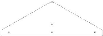
K01 PEAK TRIM - W4L20314 (x1) 5/8"x5 1/4"x16 9/16" (16x134x420)
