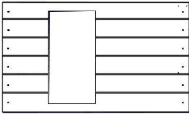
WP07 WALL PANEL - W2A04382 (x2) 1 1/16"x22 1/8"x31 9/16" (27x563x802)
