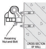
Drawing 6: Insert awning to bracket as shown in 6.1. Fix the awning with delivered safety screw, flat washer and nut (6.2) and tighten it properly.
