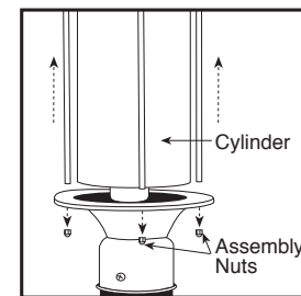
Figure 5 Cylinder Fixtures
