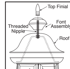
Figure 3 Harp Assembly
