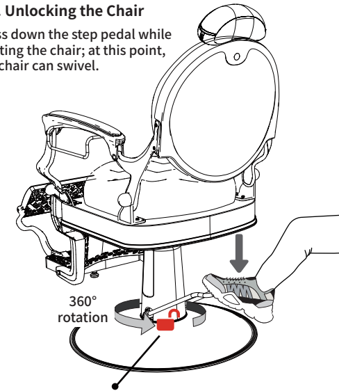
rotating unlocked
