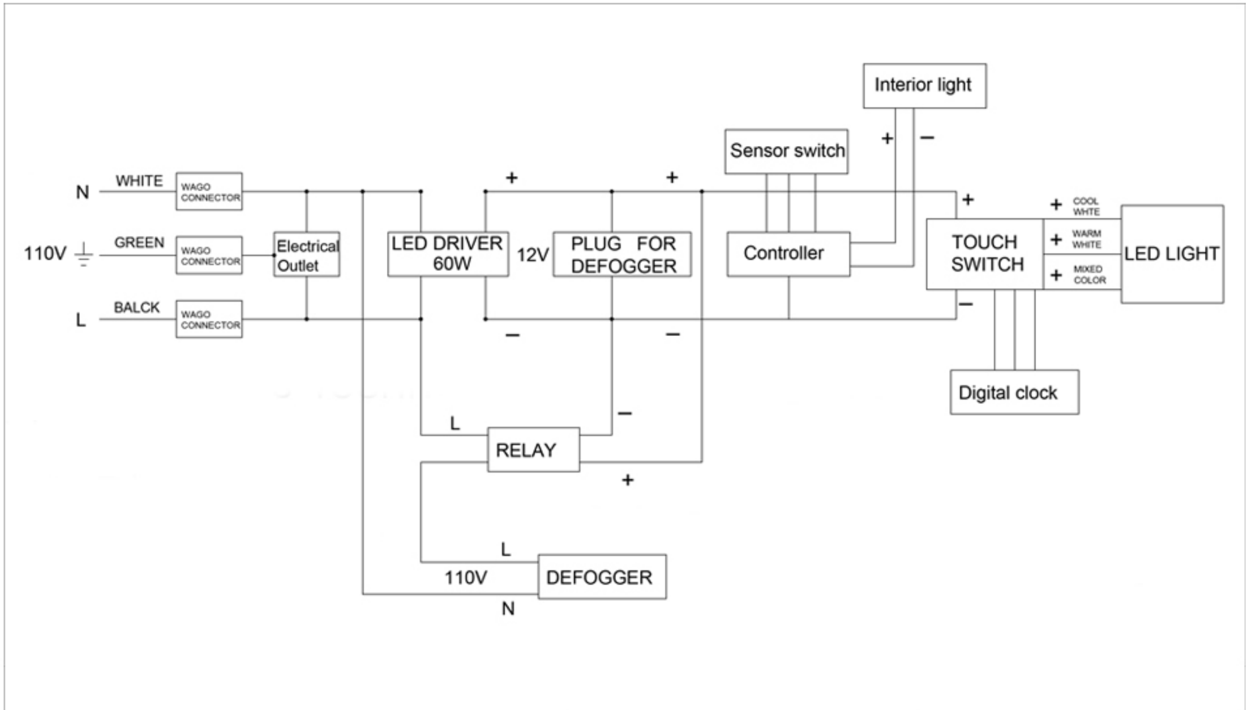
Circuit Diagram
