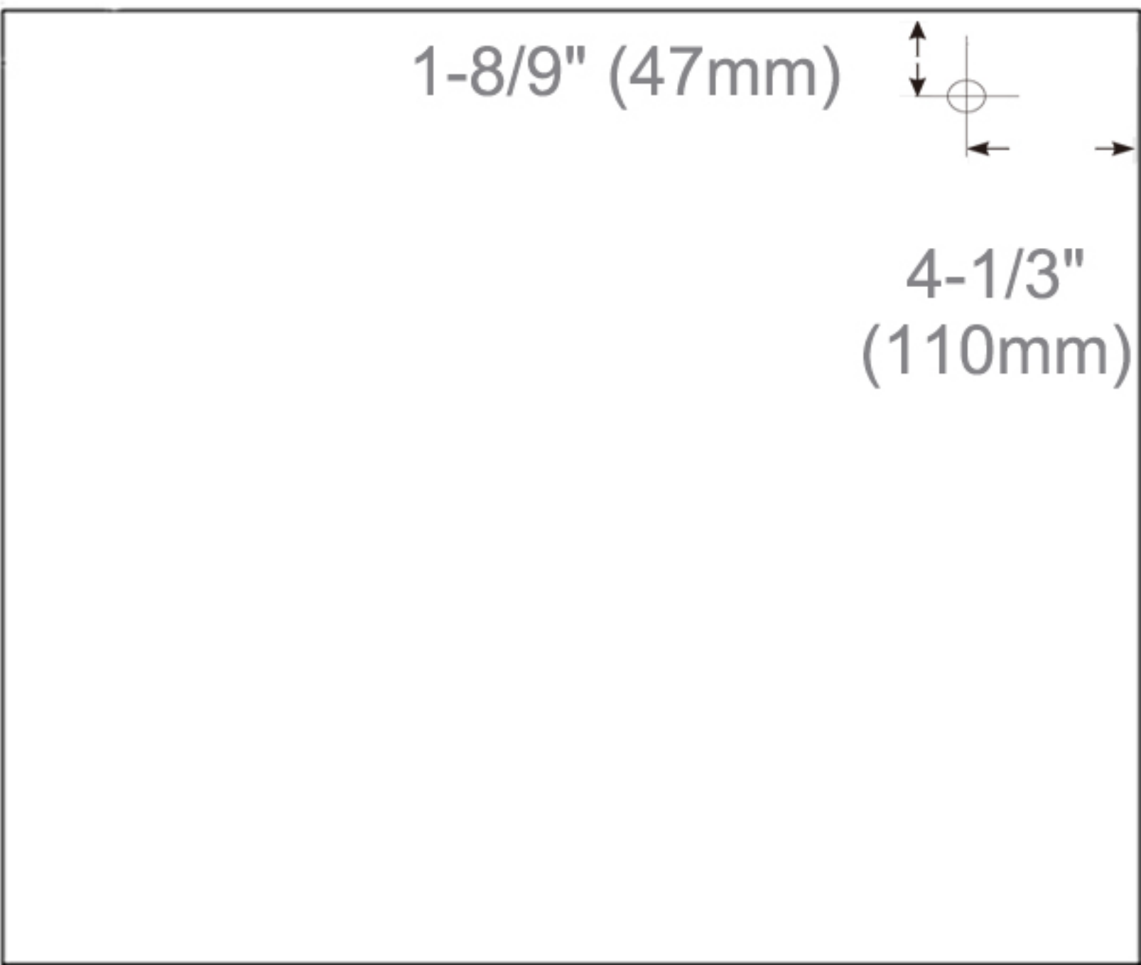
Back of Cabinet - Wire Access Location
