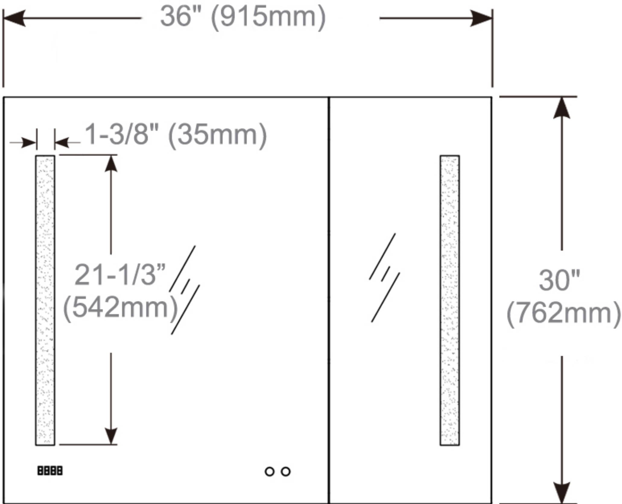
Cabinet Dimensions
