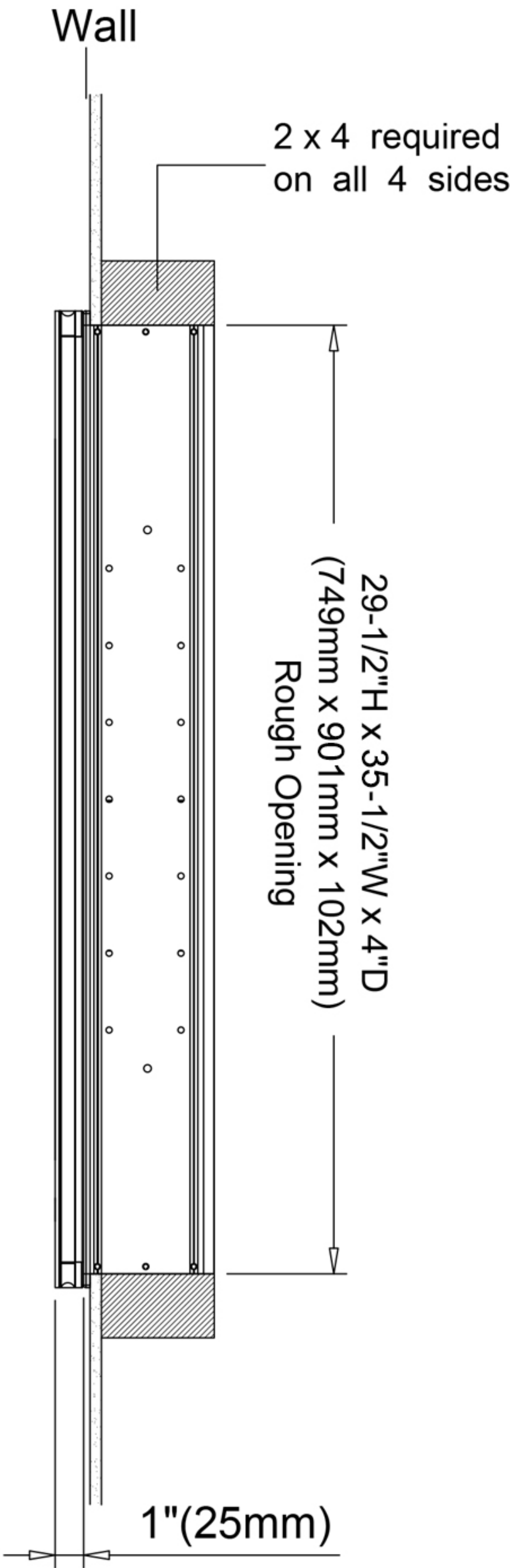
Recessed Mount
