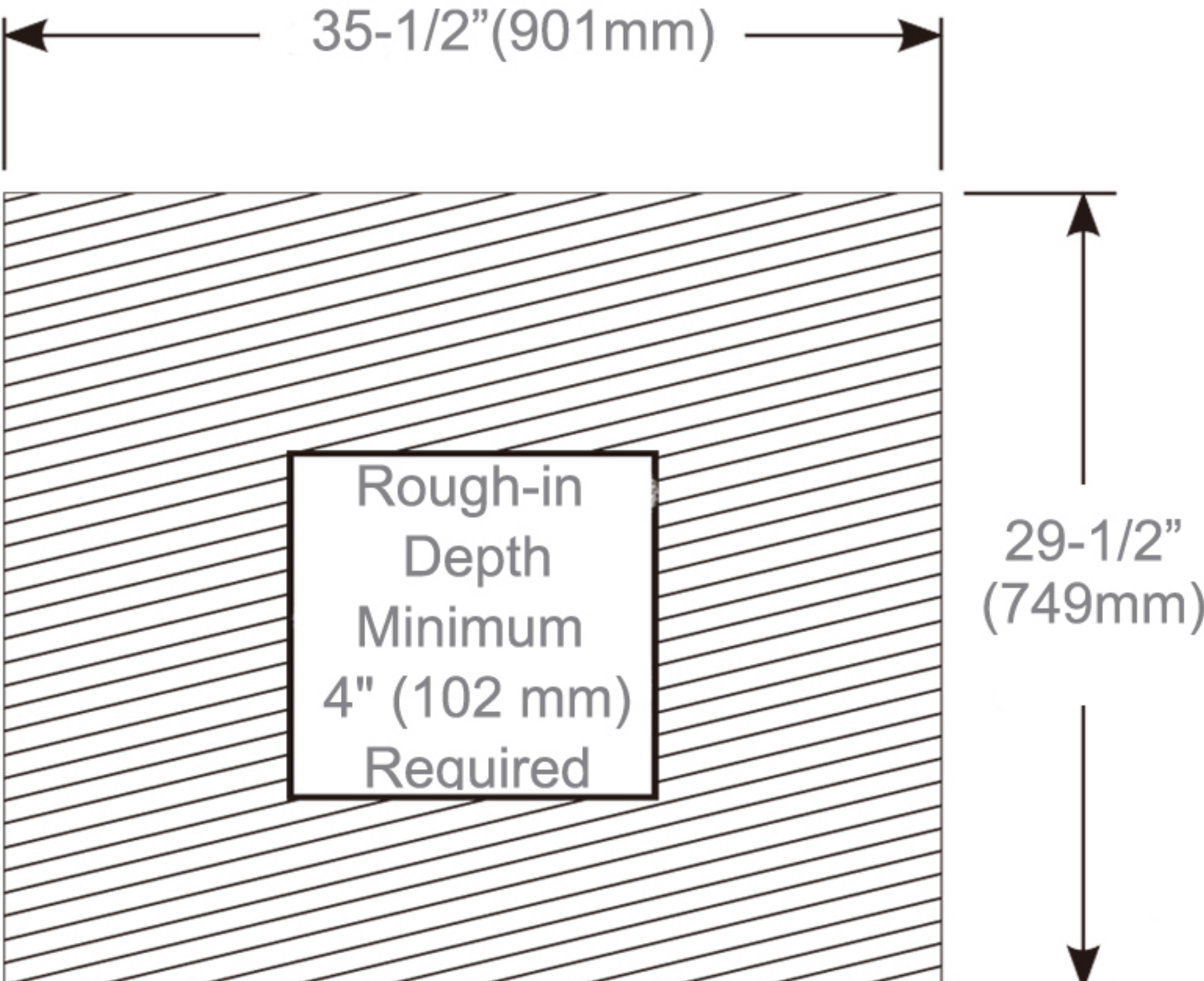
Rough-in Dimensions
