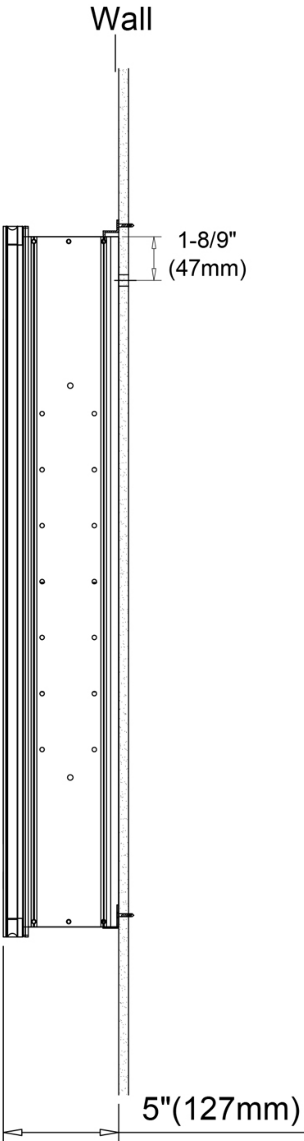
Surface Mount
