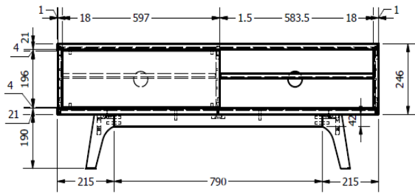
FRONT VIEW TAMPAK DEPAN
