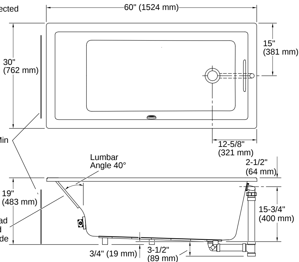
1-1/2" Bath Drain
