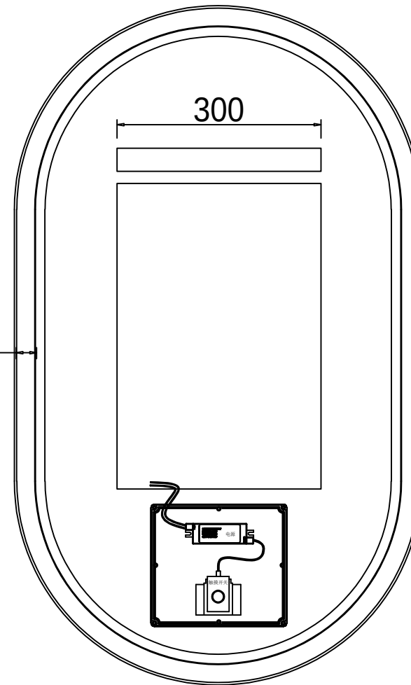
rear view
