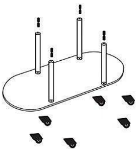
install the wheel with NO.1 screw and turn the NO.2 connecting rod on the post
