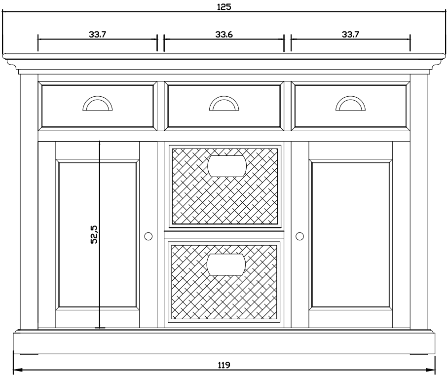
FRONT VIEW
