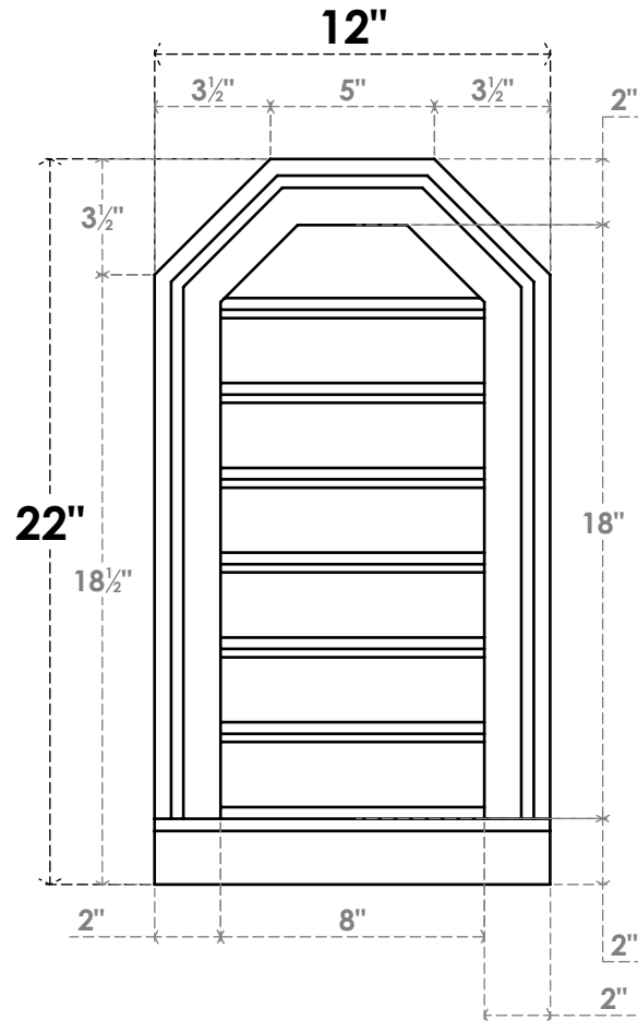
FRONT
