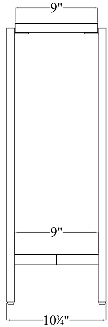
SIDE VIEW
