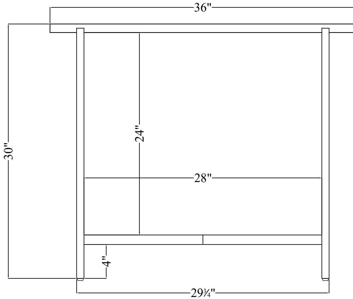
FRONT VIEW
