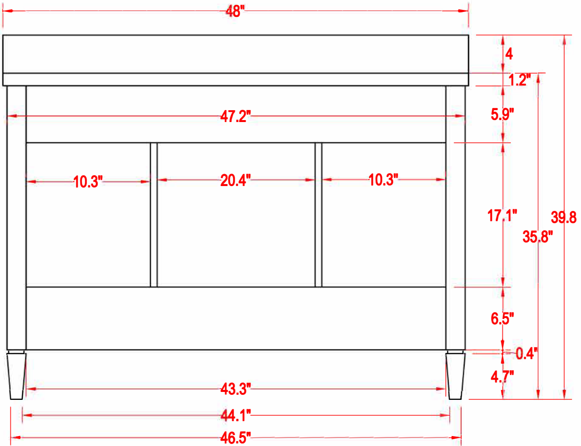
(BACK)
