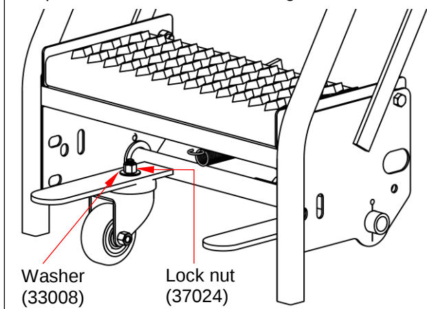
Step 4: Fasteners installed and tightened
