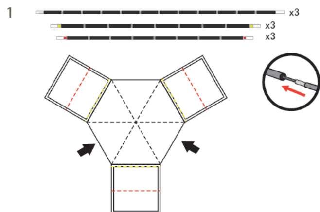
1. Assemble the poles and push them through the sleeves on the outside of the flysheet.
