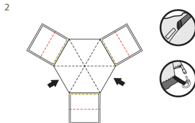
2. Insert the metal tips onto the rings of tent corners.
