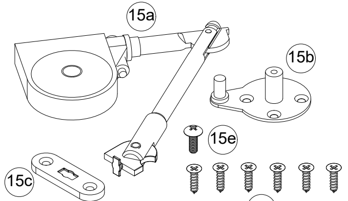
(x2) #A67750 lid stay kit
