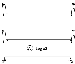
L Support bar x1
